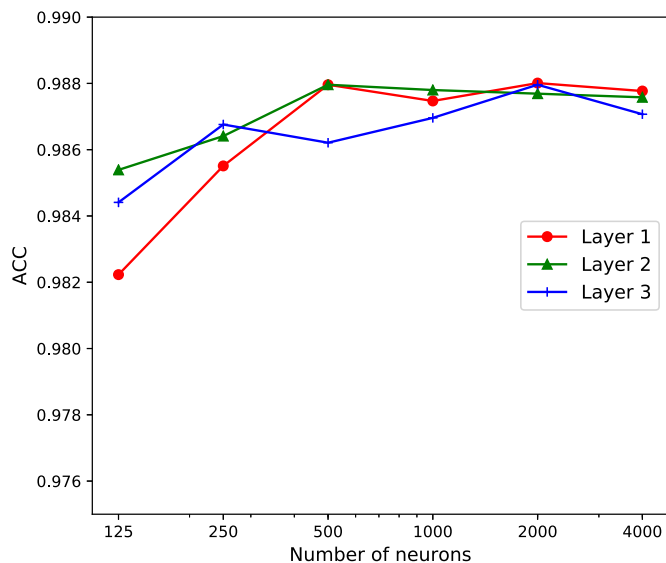
Fig. 7. Sensitivity of the network structure on MNIST-full dataset. In a wide range, the clustering accuracy is insensitive to the number of neurons of the network.
