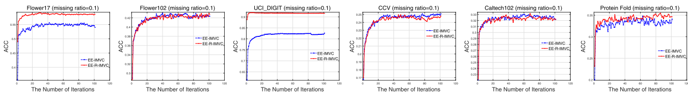
Fig. 6. The evolution of the learned consensus clustering matrix \mathbf{H} by EE- IMVC and EE- R-IMVC with missing ratio 0.1 on all datasets. The curves with other missing ratios are similar and we omit them due to space limit.
