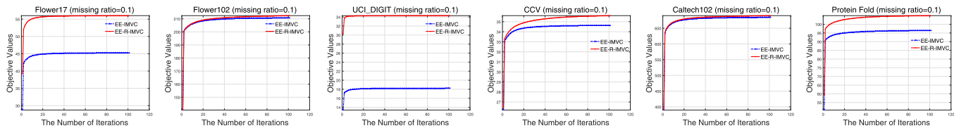
Fig. 8. The objective values of EE-IMVC and EE-R-IMVC with iterations with missing ratio 0.1 on all datasets. The curves with other missing ratios are similar and we omit them due to space limit.
